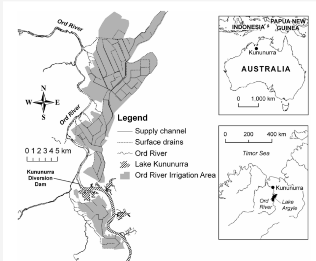
Figure 2: Location of the ORIA in northern western Australia
