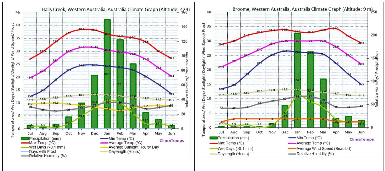
Figure 5: Climographs of Halls Creek and Broome, Australia. Sources:
