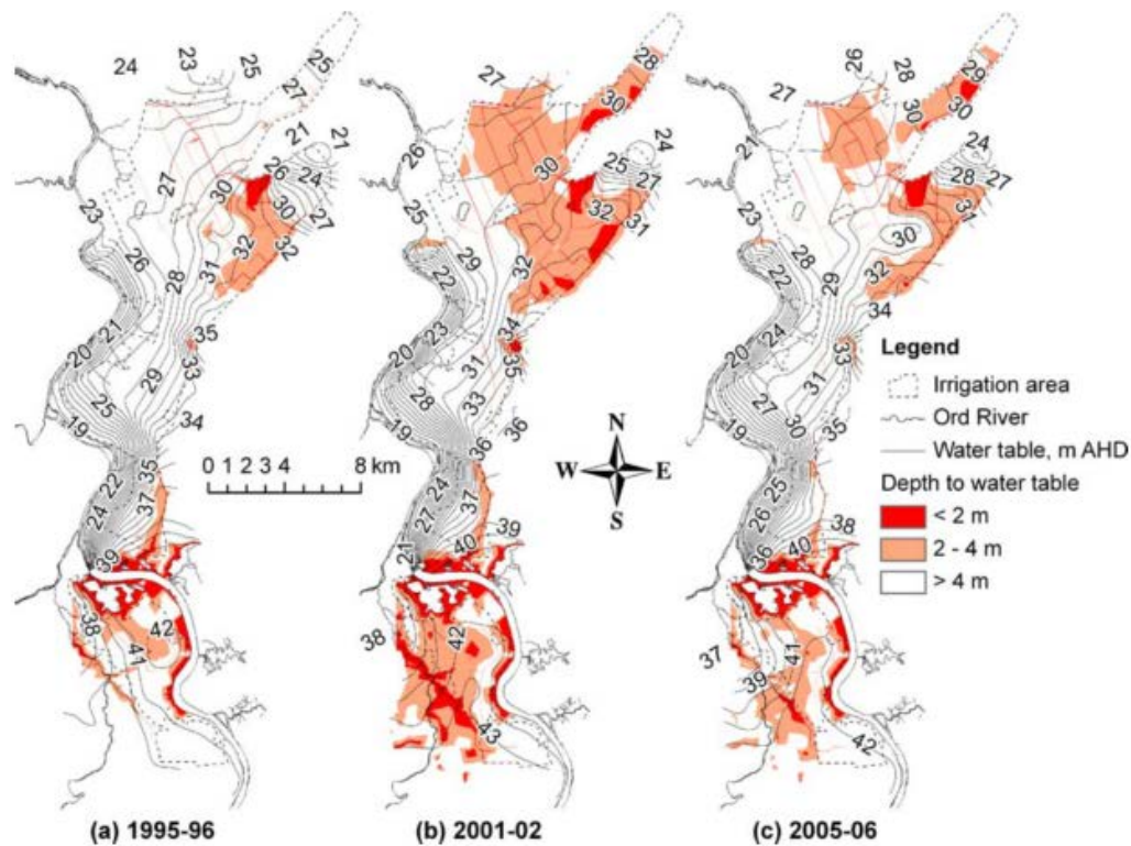
Fig. 2 Interpolated depth below ground of the mean annual water table: a July 1995 to June 1996, b July 2001 to June 2002, c July 2005 to June 2006. Contours are based on water level measurements from 65 monitoring sites
