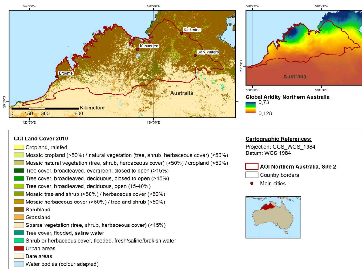
Figure 4: Overview of test site 02, Northern Australia, showing land cover from the CCI Land Cover data set on the left-hand side and an aridity index map on the right-hand side derived from the CGIAR-CSI global aridity data base.
