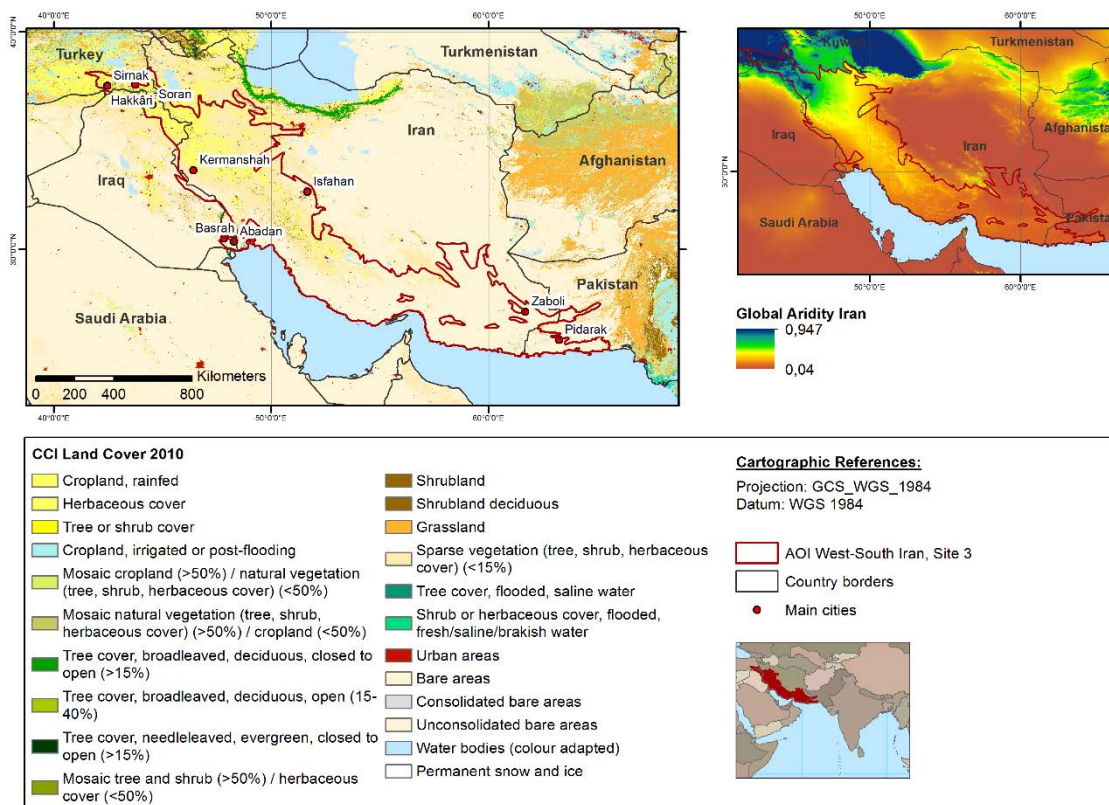
Figure 3: Overview of test site 03, South-West Iran West, showing land cover from the CCI Land Cover data set on the left-hand side and an aridity index map on the right-hand side derived from the CGIAR-CSI global aridity data base.
