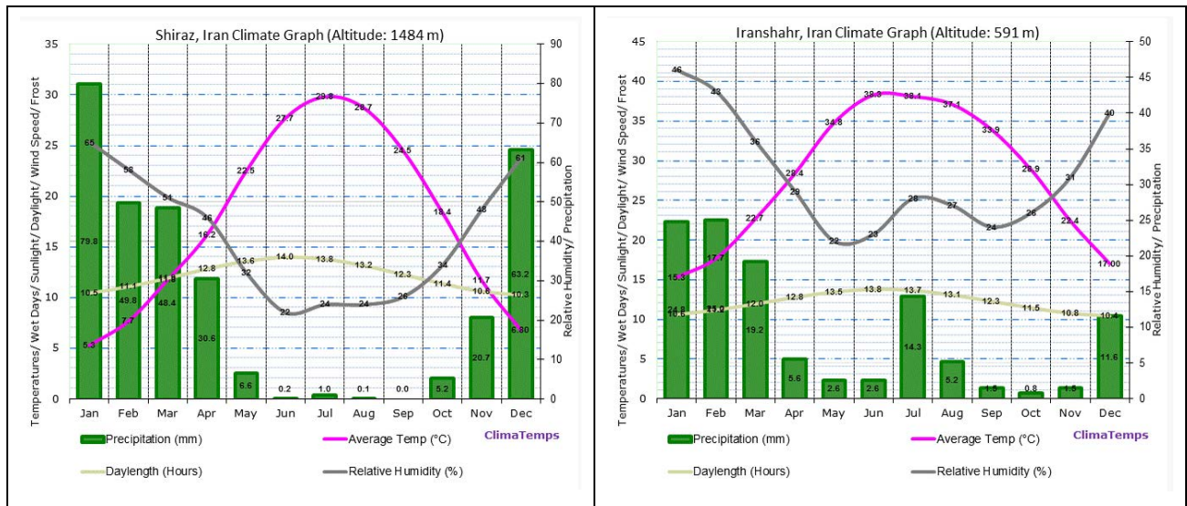
Figure 4: Climographs of Shiraz and Iranshahr. Sources:
