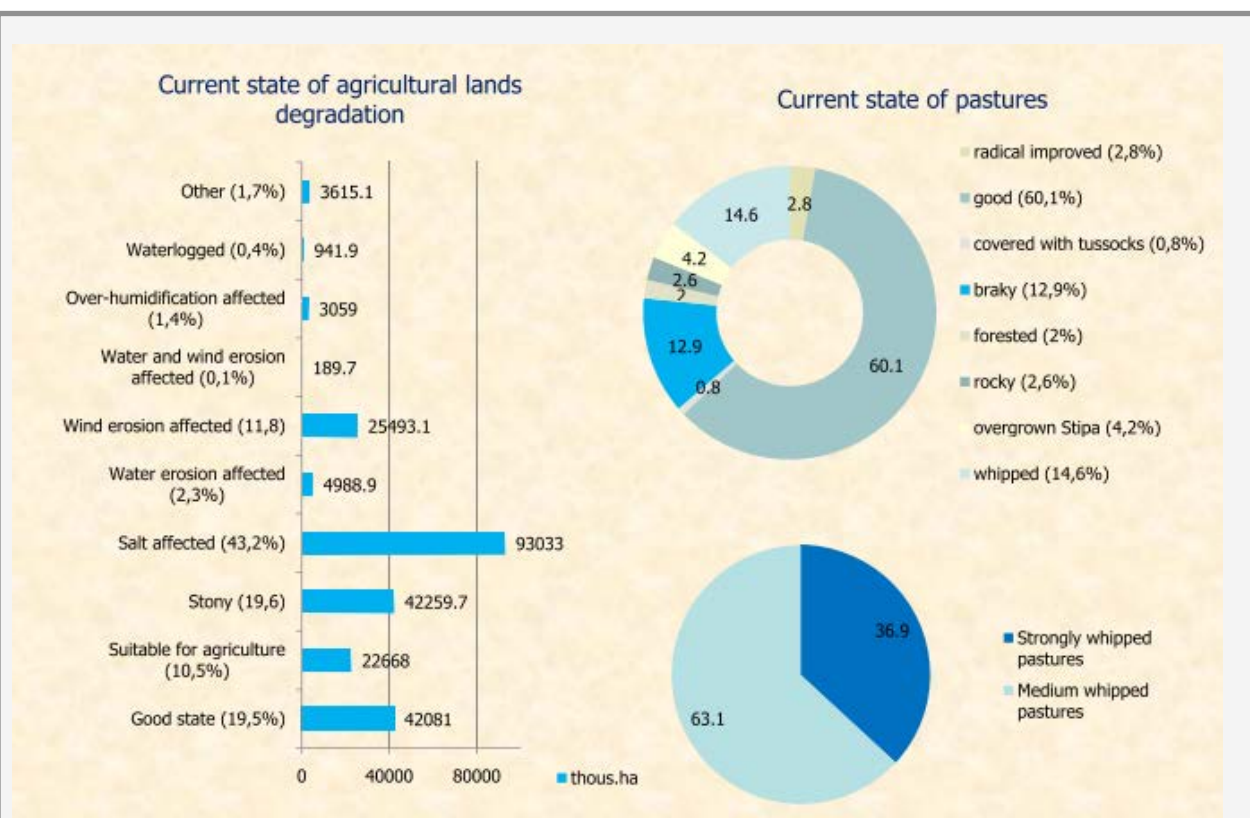
Figure 3: State of agricultural lands degradation and state of pastures (LADA 2011)
