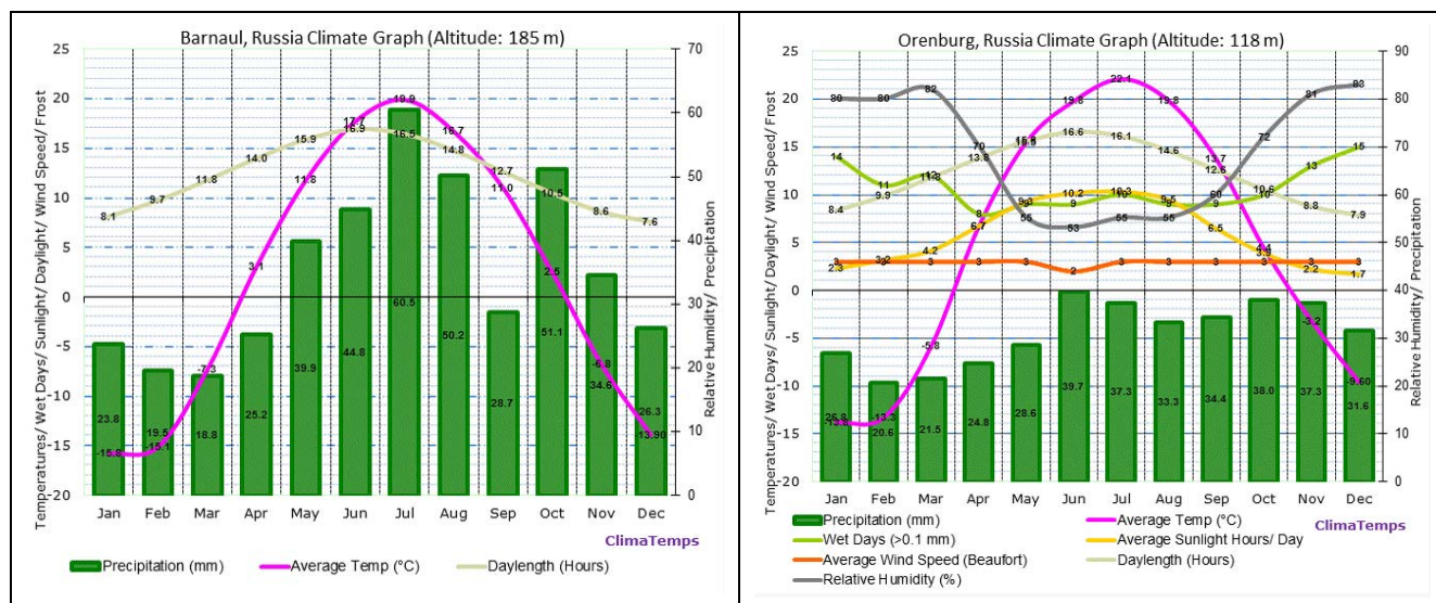
Figure 5: Climographs of Barnaul and Orenburg, Russia. Sources:
