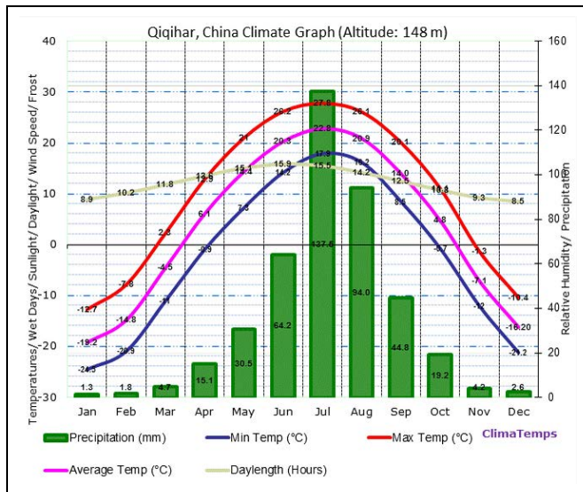
Figure 6: Climographs of Qiqihar, China. Source:
