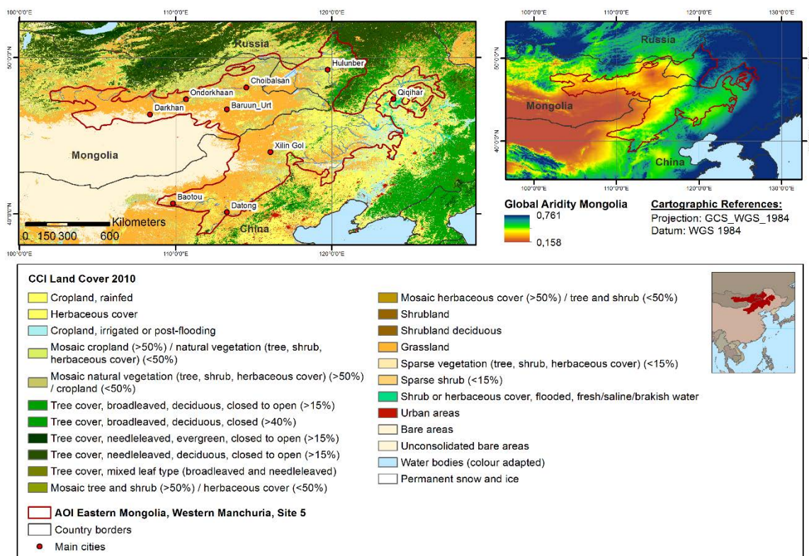
Figure 5: Overview of test site 05, Eastern Mongolia and Western Manchuria, showing land cover from the CCI Land Cover data set on the left-hand side and an aridity index map on the right-hand side derived from the CGIAR-CSI global aridity data base.
