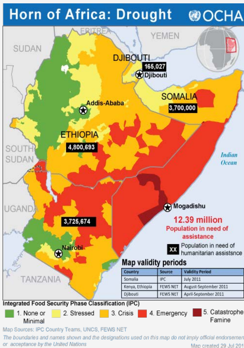
Figure 2: Drought and Food Security at the Horn of Africa, source:
