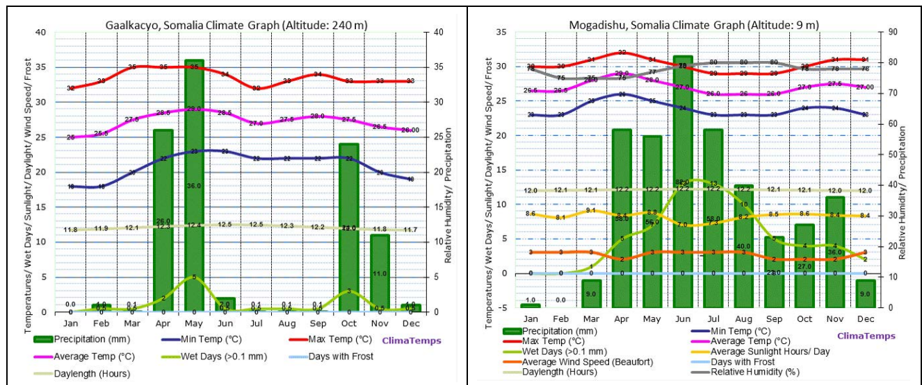
Figure 4: Climographs of Gaalkacyo, central Somalia, and Mogadishu, southern Somalia. Sources:
