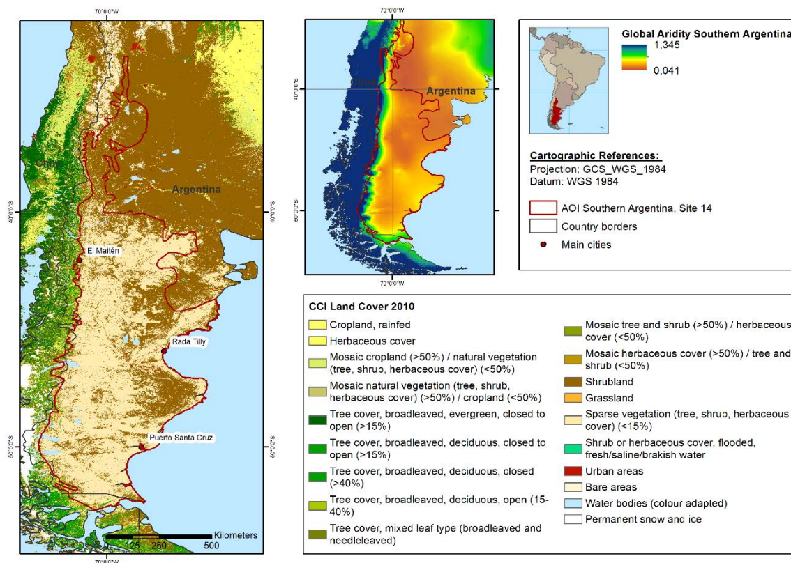
Figure 3: Overview of test site 14, Southern Argentina, showing land cover from the CCI Land Cover data set on the left-hand side and an aridity index map on the right-hand side derived from the CGIAR-CSI global aridity data base.
