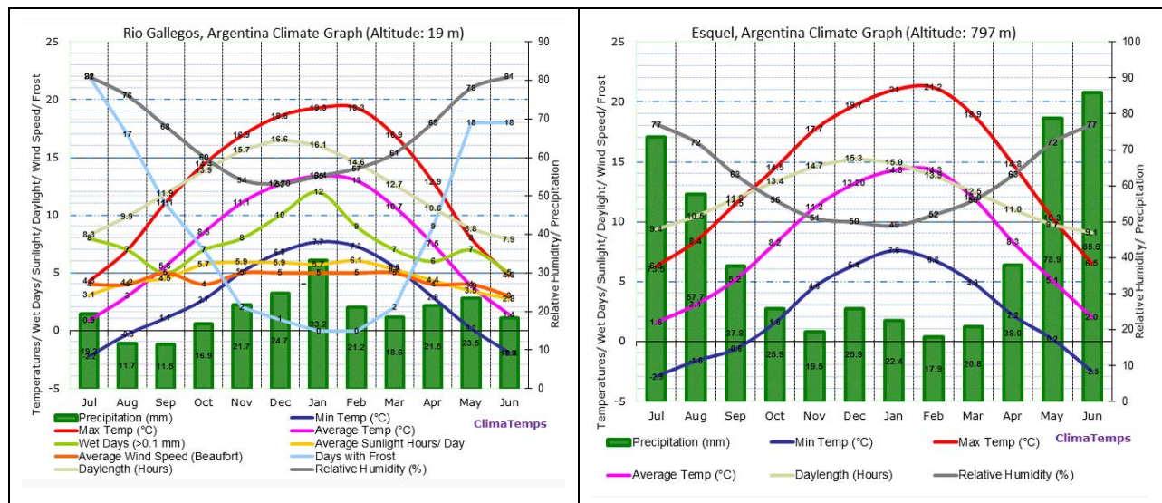
Figure 4: Climographs of Rio Gallegos and Esquel, Argentina. Sources: http://www.rio-gallegos.climateemps.com/ , http://www.esquel.climateemps.com/
