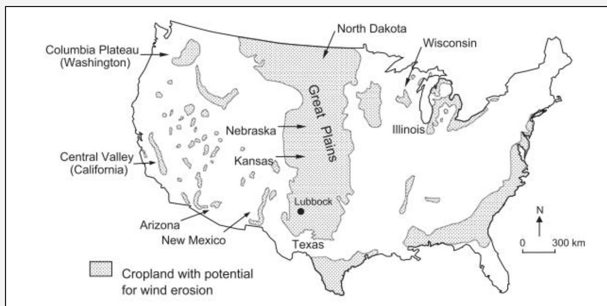
Figure 3: Locations of cropland areas of the USA threatened by wind erosion
