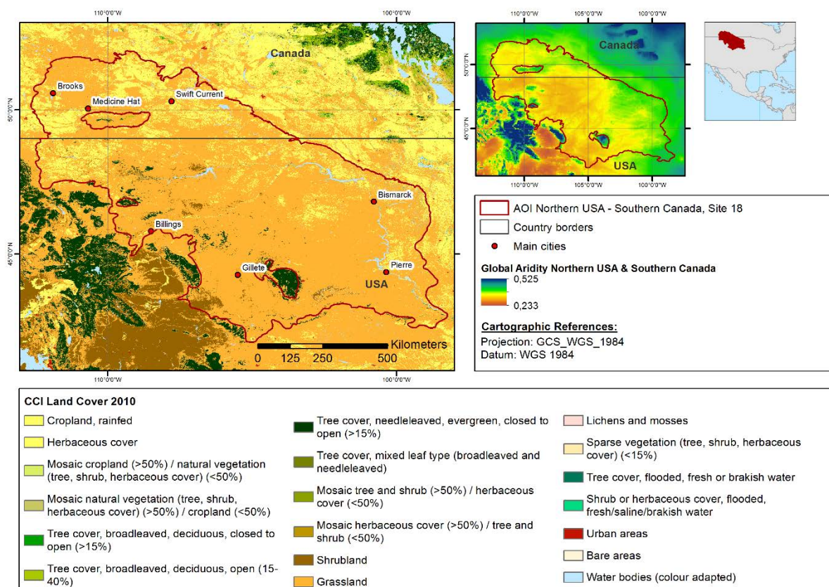
Figure 4: Overview of test site 18, Northern USA - Southern Canada, showing land cover from the CCI Land Cover data set on the left-hand side and an aridity index map on the right-hand side derived from the CGIAR-CSI global aridity data base.
