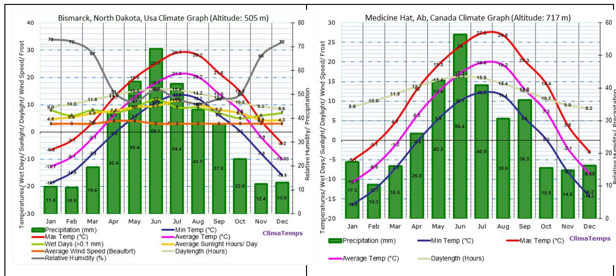
Figure 5: Climographs of Bismarck, North Dakota and Medicine Hat, Alberta. Sources:
