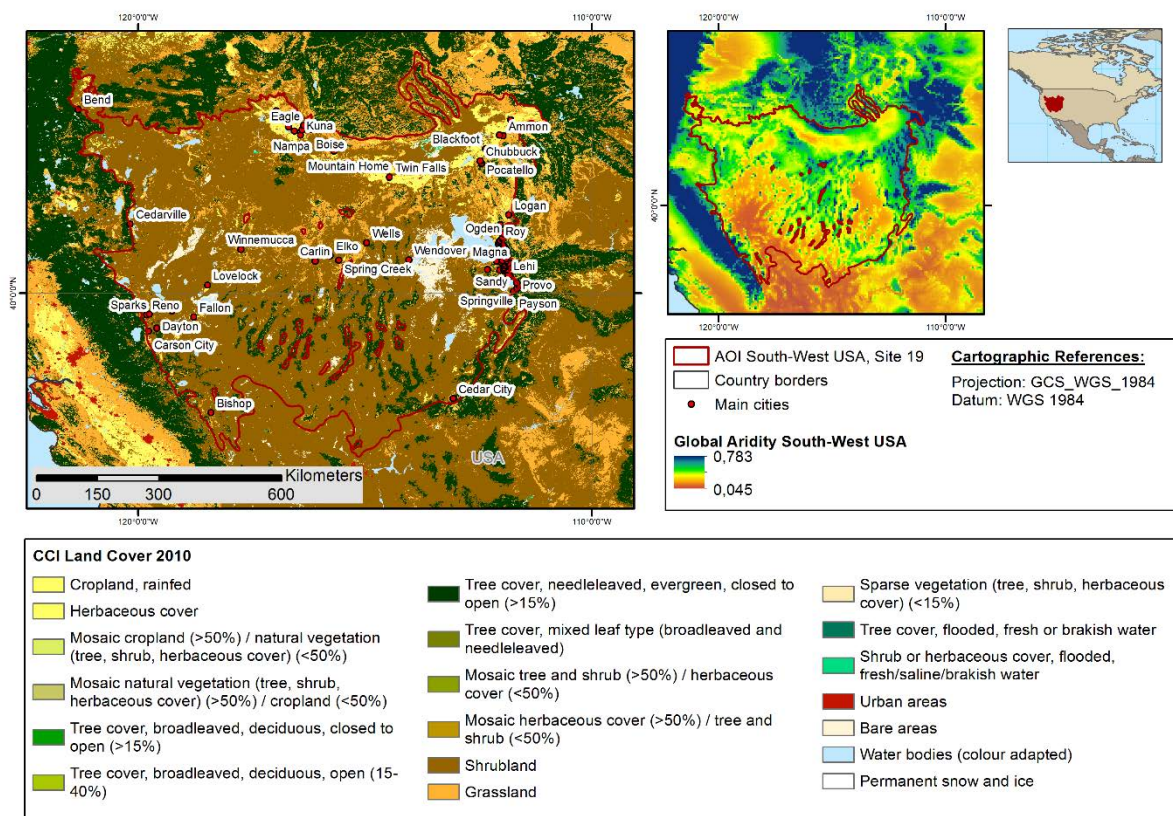
Figure 4: Overview of test site 19, South West USA, showing land cover from the CCI Land Cover data set on the left-hand side and an aridity index map on the right-hand side derived from the CGIAR-CSI global aridity data base.
