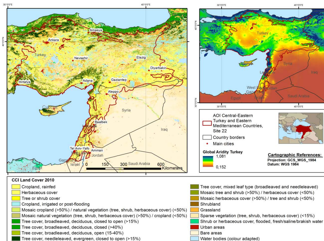
Figure 3: Overview of test site 22, Eastern Mediterranean Countries, showing land cover from the CCI Land Cover data set on the left-hand side and an aridity index map on the right-hand side derived from the CGIAR-CSI global aridity data base.
